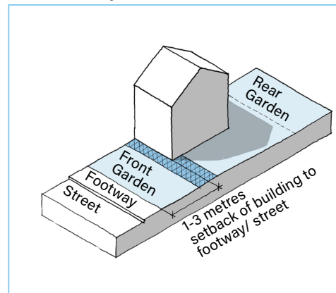
Fig B.7 Frontage setbacks from footway/ street.
