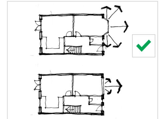
Fig M.8 Use bay windows or other projections to create greater and more effective outlook.
