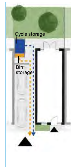
Fig B.24 Refuse and cycle storage to rear of a car port.
