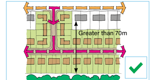
Fig B.79 Sufficient plot depth maintaining front to front and back to back relationships on the edge of existing plots.
