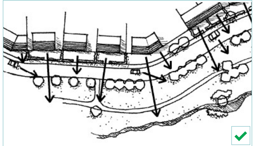
Fig N.10 Use buildings to provide enclosure and natural surveillance over adjacent open space.
