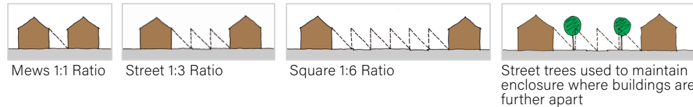
Fig M.13 Acceptable height to width ratios.
