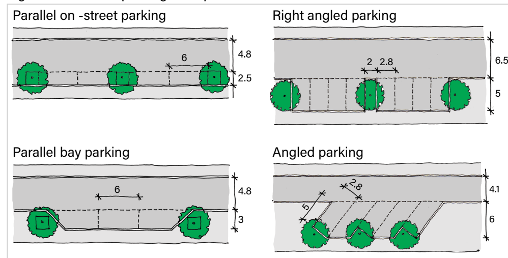
Fig M.15 On street parking examples.
