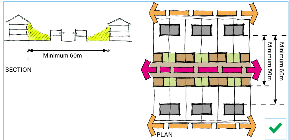
Fig B.83 Courtyard or frontage infill development.
