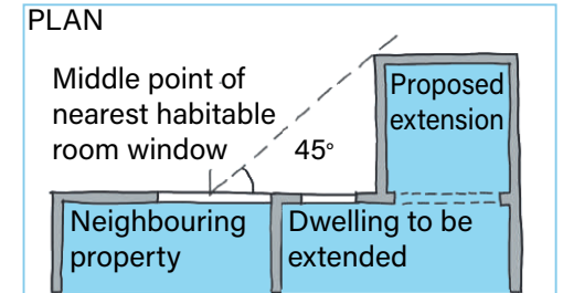
Fig B.49 The 45° rule: The proposed extension should not project beyond the '45° line' (indicated by the dashed line) into the neighbours protected area.
