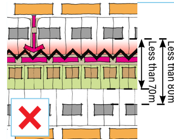
Fig B.75 Without sufficient plot depth, the fronts of new houses compromise the privacy and security.
